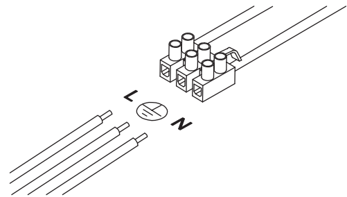
4. Connect the wires
