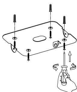
3. Drill holes & apply plastic anchors With screws
