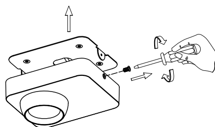
2. Untight the side screws
