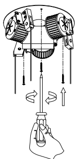
3. Drill holes & apply plastic anchors With screws
