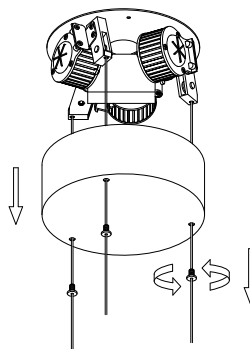
2. Untight the screws & remove the canopy
