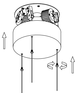
5. Tight the screws up & Place the canopy in place
