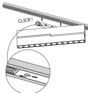
2. Click the product in to place
