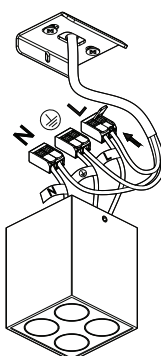
5. Connect the wires
