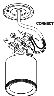
5. Connect the wires
