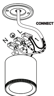
5. Connect the wires
