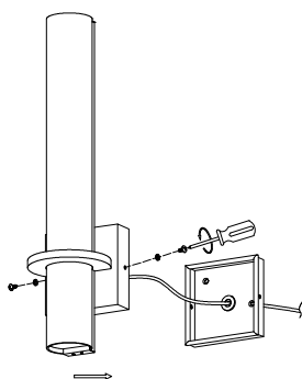
5. Apply the Side screws
