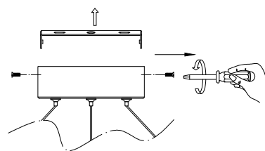
2. Untight the side screws
