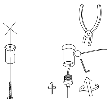
4. Fix in place the hanging element
