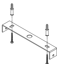
3. Apply the plastic anchors With the screws
