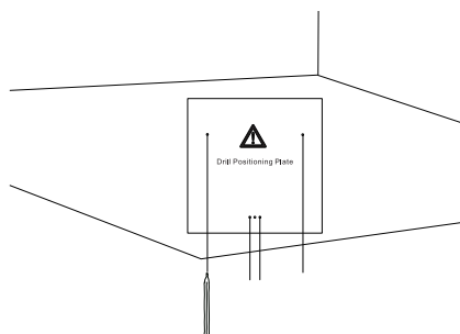
Mark holes
