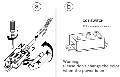
Connect assisting cords
