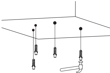
Apply plastic anchors
