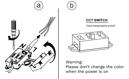
Connect assisting cords
