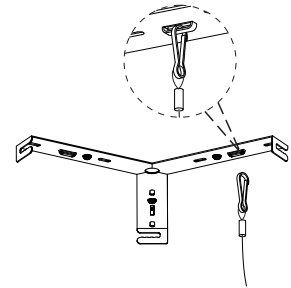
Connect assisting cords
