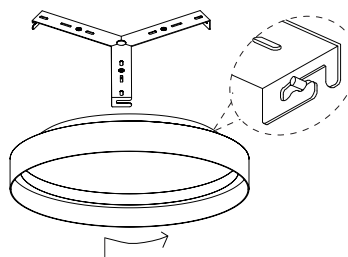
Apply it on place by clicking it into the openings
