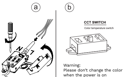
Connect the wires
