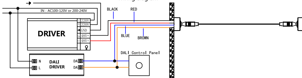
Wiring diagram
