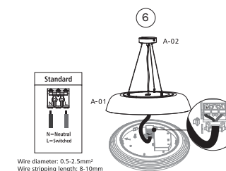
Connect wires
