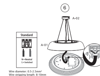
Connect wires
