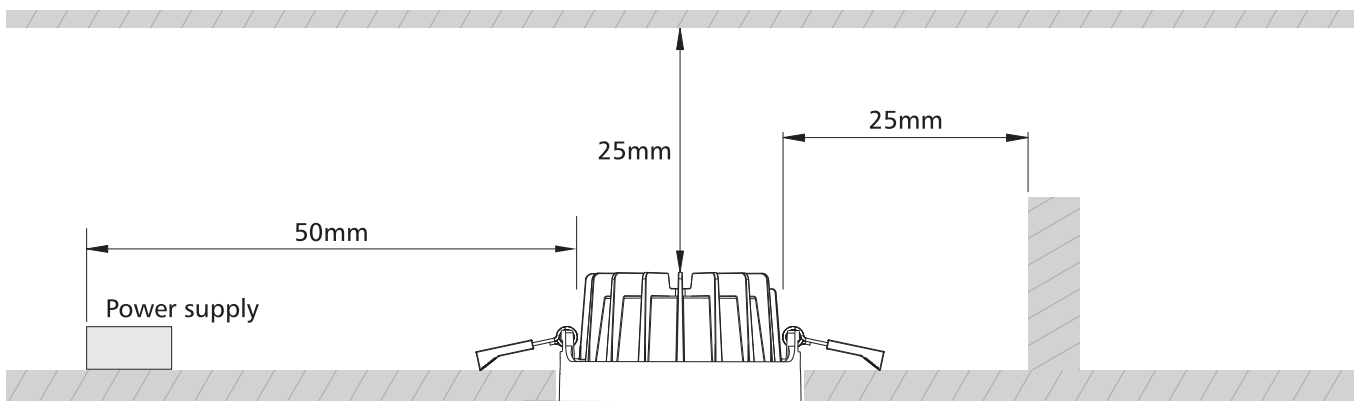
Fig 1: Installation Spacing
