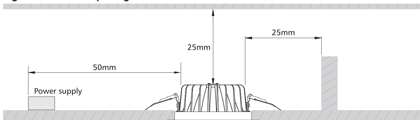
Fig 1: Installation Spacing
