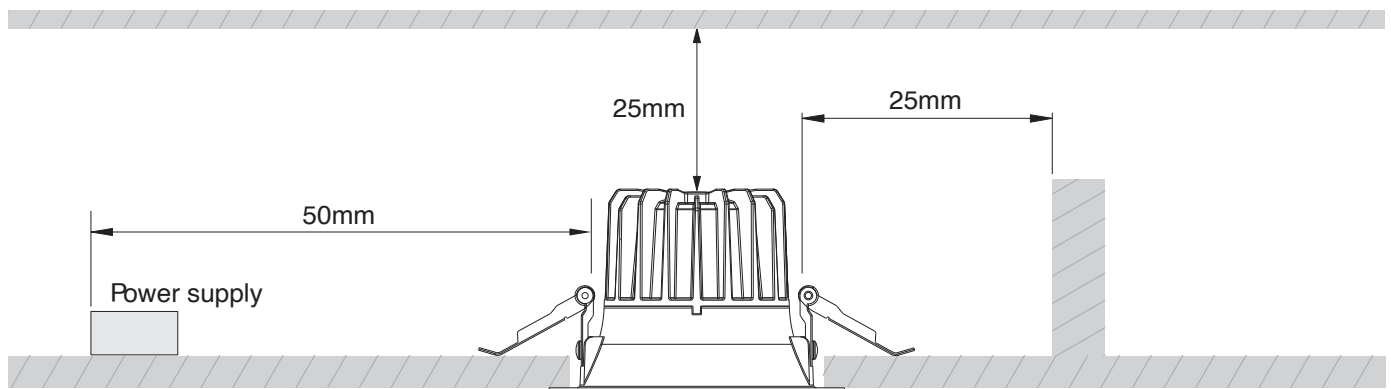
Fig 1: Installation Spacing
