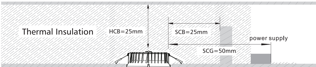
Fig 1: Installation Spacing
