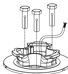
4. Apply the screws
