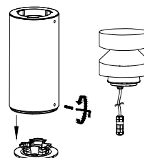
2. By rotating, break it apart
