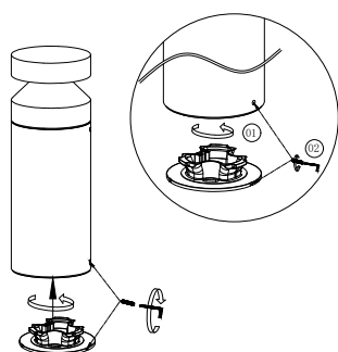
7. Put it in place and apply the side screw
