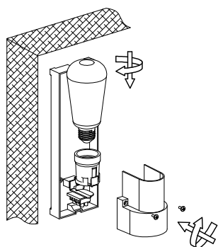
5. Insert the bulb by tiding it in place & apply screws to connect the cap
