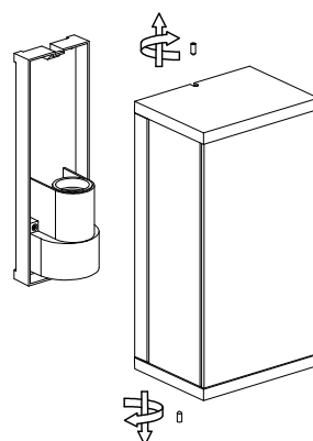
2. Untie side screws to remove the cap
