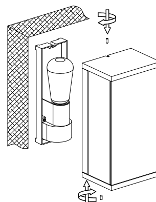
6. Apply the cap by tiding up the side screws
