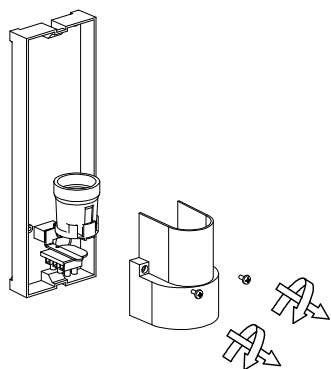
3. Untie screws to remove the rest of the parts
