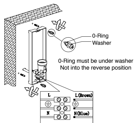
4. Connect wires & make base stable by tiding up the screws
