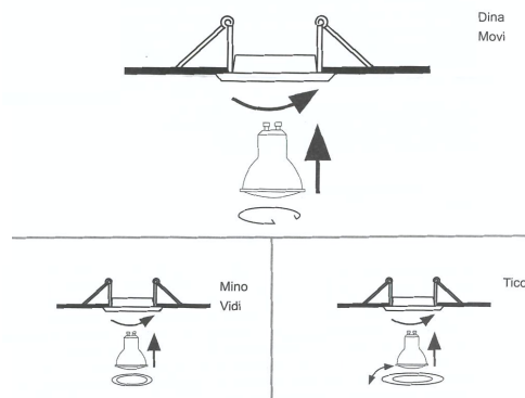
6. Insert the bulb
