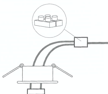
3. Connect wires
