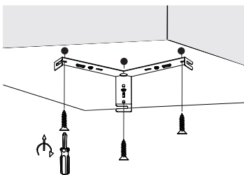
5. Apply screws
