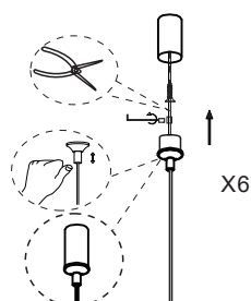
8. Adjust the wire & fix it into place
