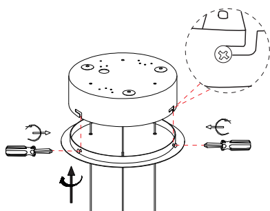
7. Apply side screws and make Hanging elements stable
