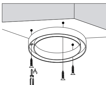
5. Apply screws
