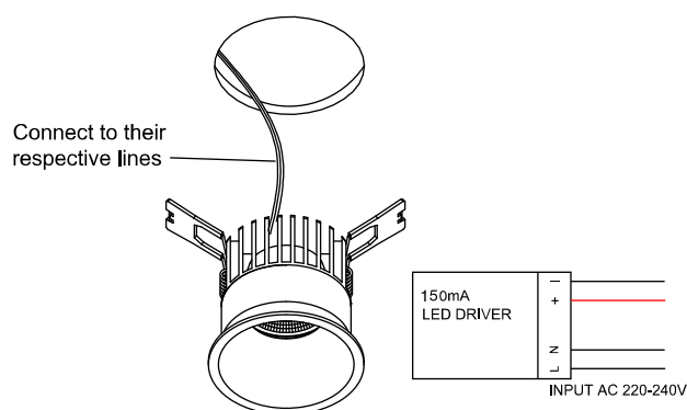
5. Connect wires of the driver
