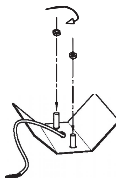
4. Apply the top screws
