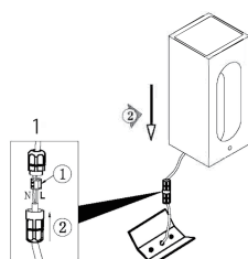
5. Connect the wires
