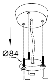
Drill holes & apply the nuts
