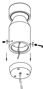
Apply the side screws
