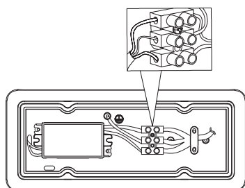
7. Place the cables in to place
