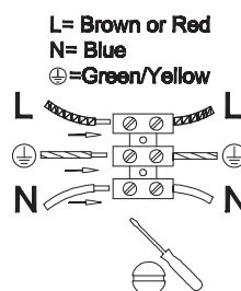
6. Connect the wires
