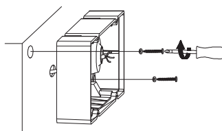
5. Apply the screws
