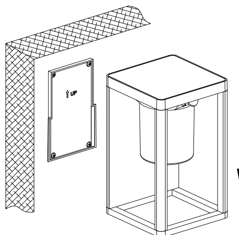
4. Place the lamp into the base from the way up downwards
