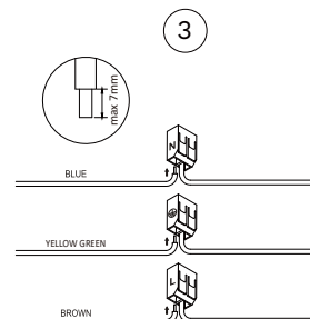
Connect the 3 wires
