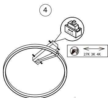
Apply the side screws
