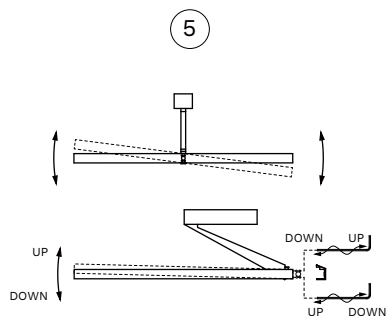
Adjust the lamp body to a horizontal position
