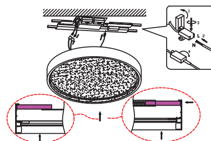
Connect wires
