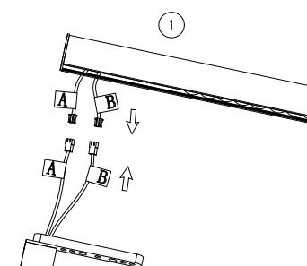
Connect wires as marked
