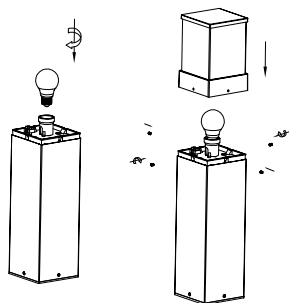
10. Install the bulb, apply the cap With the side screw
