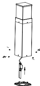
8. Tight the side screws
