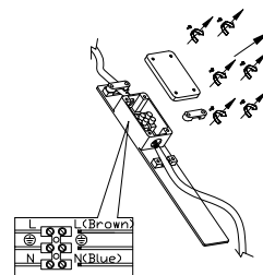
3. Untight the screws to Connect the wires
