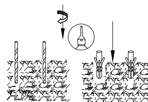
6. Drill on the marked areas & Apply plastic anchors
