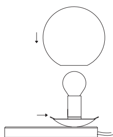
3. Press the clip to the inside & apply the glass
