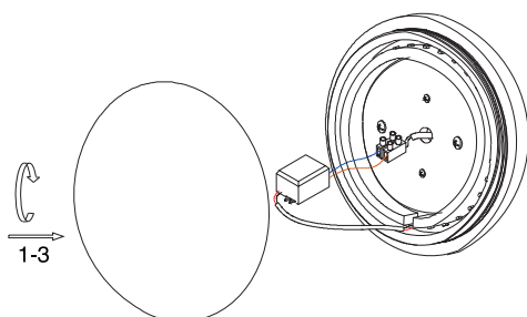
3 Connect the wires and apply the Side screws
