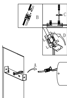
5 Connect the wires
