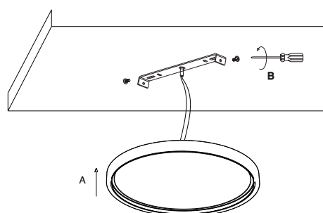
6 Apply the side screws
