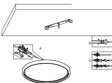
5 Connect the wires
