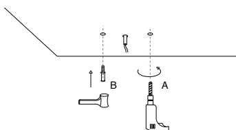
3 Apply plastic anchors
