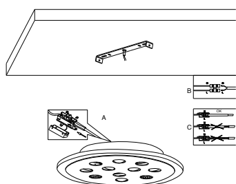
5 Connect the wires
