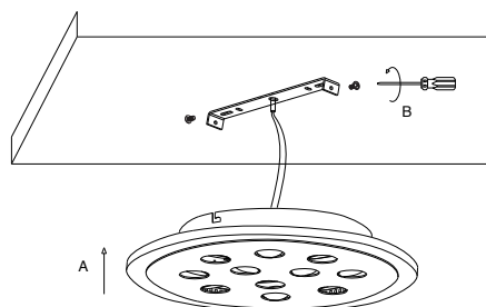
6 Apply the side screws
