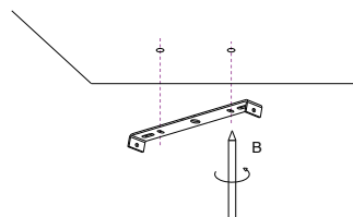
2 Align, where holes should be
