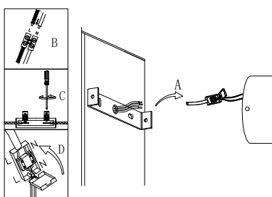
5 Connect the wires
