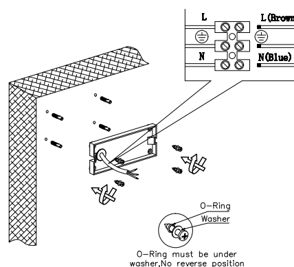
4. Apply screws & connect screws
