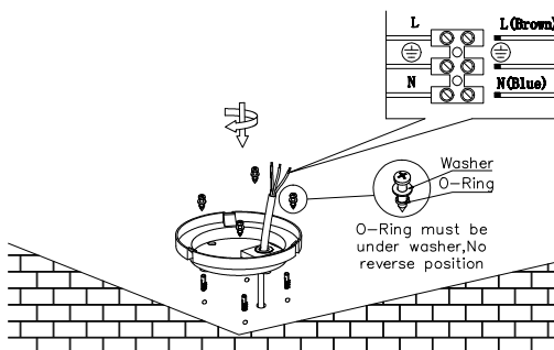
3. Install cable, tie up screws & connect the wires
