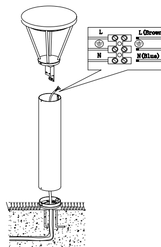
4. Connect wires
