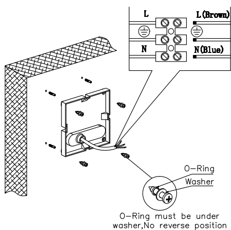
3. Tie up screws & connect wires
