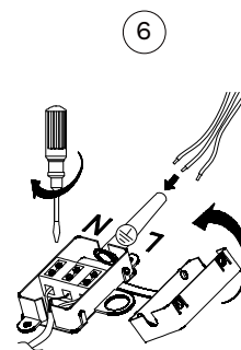
Connect the wires
