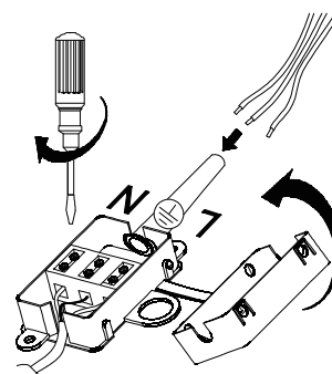
6. Connect the wires
