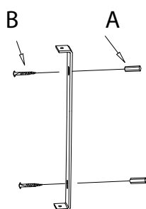
3. Apply plastic anchors with screws
