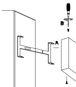
5. Apply the side screws
