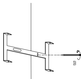
2. Mark & drill holes
