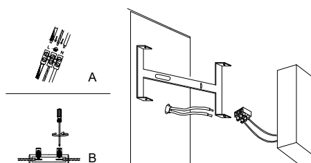
4. Connect the wires
