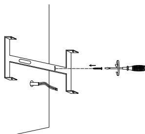
3. Apply plastic anchors with screws
