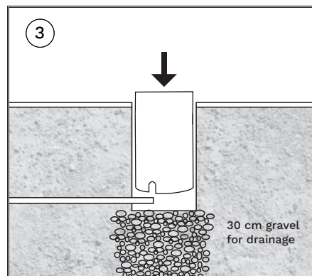
Install the PVC tuber into position
