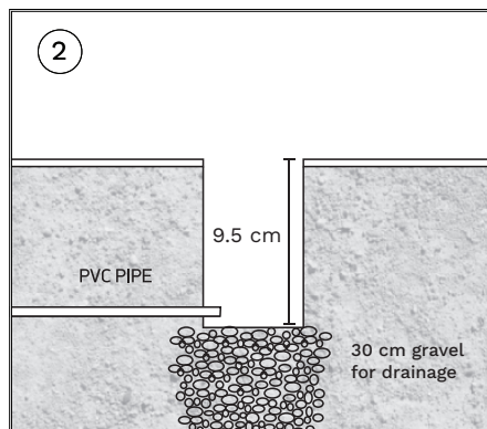
Prepare for installation by applying 30 cm layer of gravel for drainage
