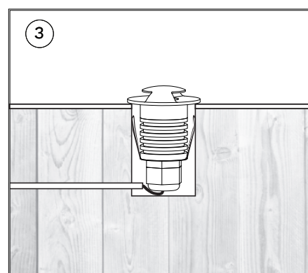
Fix it into place
